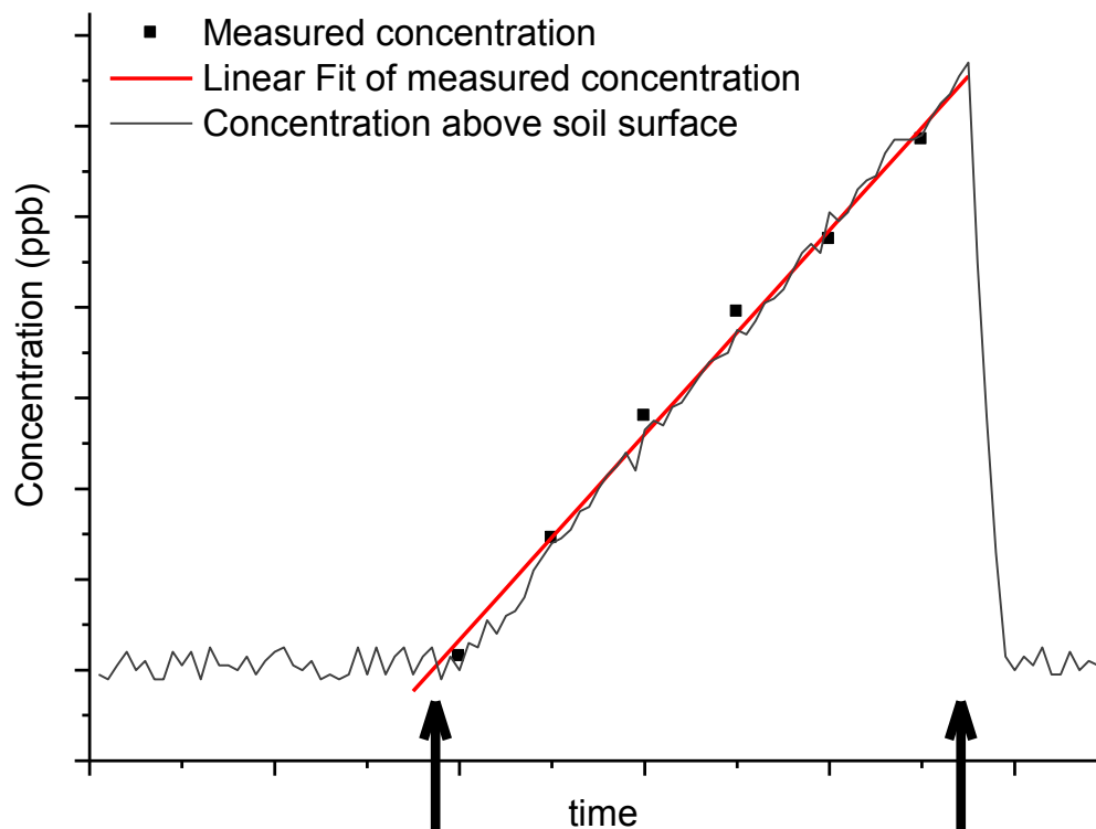
Fig. 2 Theoretical evolution of the concentration of a gas being emitted from the soil upon use of a static chamber. Concentration of the gas above the soil surface (black line) remains at a relatively constant level; at the moment when the chamber is closed (left arrow), the concentration in its headspace begins to rise. Along the closing period of the chamber, several gas samples are taken (black squares) and subsequently the concentration is determined, e.g. by use of gas chromatography. Right after opening the chamber (right arrow) concentration above soil surface returns to atmospheric background levels. Soil GHG emissions are most commonly calculated from the linear increase of the headspace gas concentration during the chamber closing period (red line), the volume of the chamber, the area of the soil covered by the chamber, as well as air temperature, air pressure and molecular weight of the molecule under investigation (see e.g. Butterbach-Bahl et al., 2011). It should be noted, that changes in gas concentration upon chamber closure can significantly deviate from linearity, showing e.g. saturation effects. In all cases it should be tested if non-linear flux calculation methods to not fit better observed changes in chamber headspace concentrations with time (see e.g. Pedersen et al., 2010)
