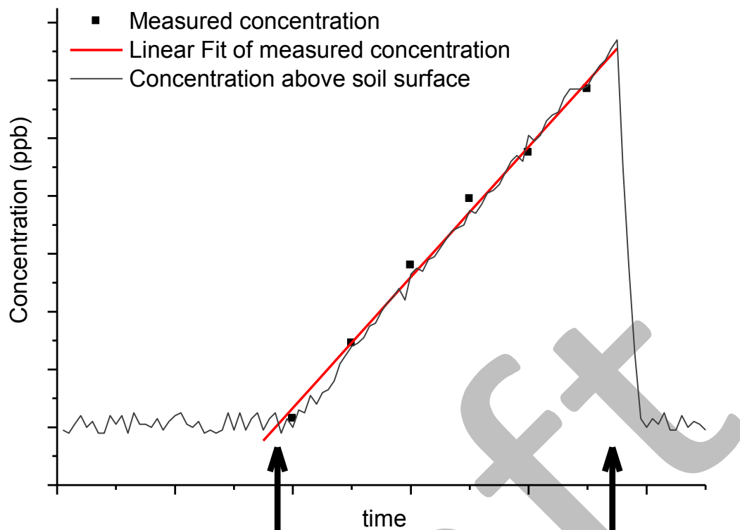
Fig. 2 Theoretical evolution of the concentration of a gas being emitted from the soil upon use of a static chamber. Concentration of the gas above the soil surface (black line) remains at a relatively constant level; at the moment when the chamber is closed (left arrow), the concentration in its headspace begins to rise. Along the closing period of the chamber, several gas samples are taken (black squares) and subsequently the concentration is determined, e.g. by use of gas chromatography. Right after opening the chamber (right arrow) concentration above soil surface returns to atmospheric background levels. Soil GHG emissions are most commonly calculated from the linear increase of the headspace gas concentration during the chamber closing period (red line), the volume of the chamber, the area of the soil covered by the chamber, as well as air temperature, air pressure and molecular weight of the molecule under investigation (see e.g. Butterbach-Bahl et al., 2011). It should be noted, that changes in gas concentration upon chamber closure can significantly deviate from linearity, showing e.g. saturation effects. In all cases it should be tested if non-linear flux calculation methods to not fit better observed changes in chamber headspace concentrations with time (see e.g. Pedersen et al., 2010)
