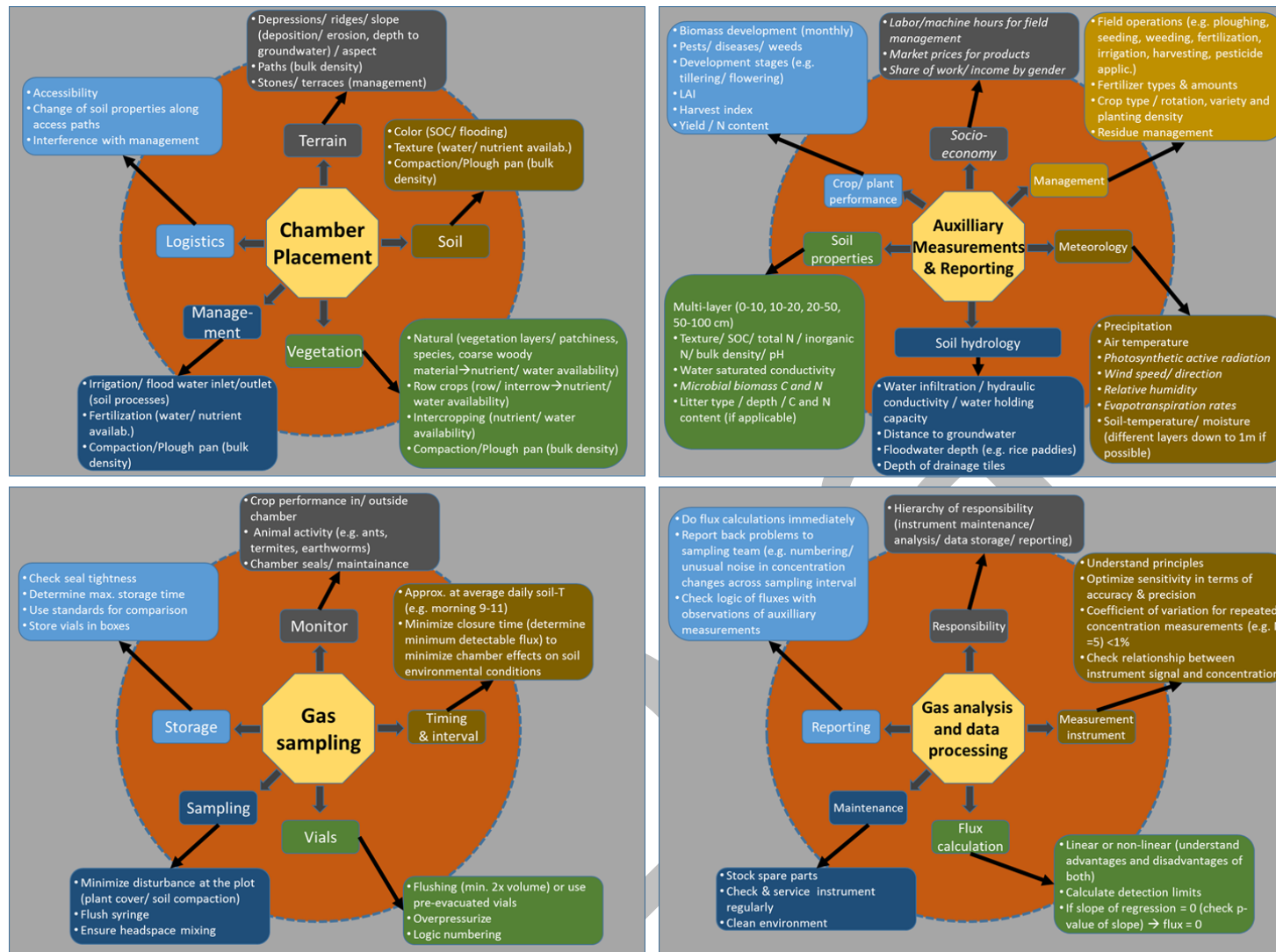
Fig. 1 General recommendations for chamber placement, gas sampling, gas concentration measurements and measurement of auxiliary parameters for static chamber soil GHG flux measurements. (Note: text in italic are additional measurements/ parameters which might be worthwhile to observe)
